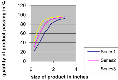
product gradation curves of impact crusher at different speeds
